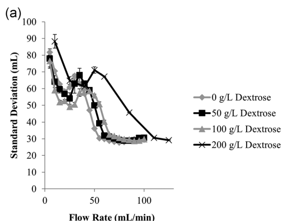
FIGURE 3 Reaction of exiting pulse injections as a function of flow rate and viscosity of mid-scale Jig in a Box (JIB) operation. (a) The pulse experiences two asymptotes and two inflection points, but at different flow rates. Error bars representing (+/-) the sample standard deviation are plotted. Data points with no error bars had a small enough difference that the dot symbol covers the bars. (b) Peak spreading is normalized along the x-axis by Equation (1) and the y-axis by Equation (3), allowing the two asymptotes and two inflection points to align
